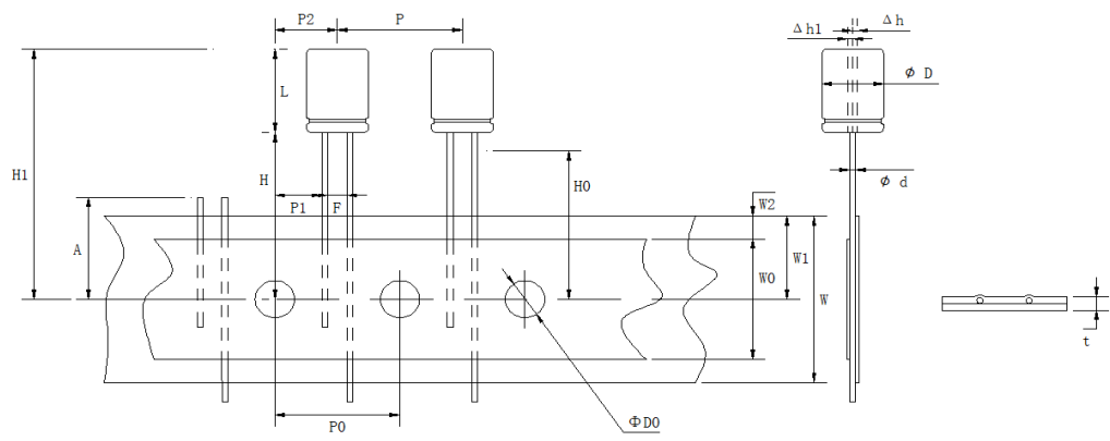
[ Fig. 4 (Diameter for Φ10 )
